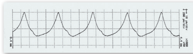
Roughness profile
